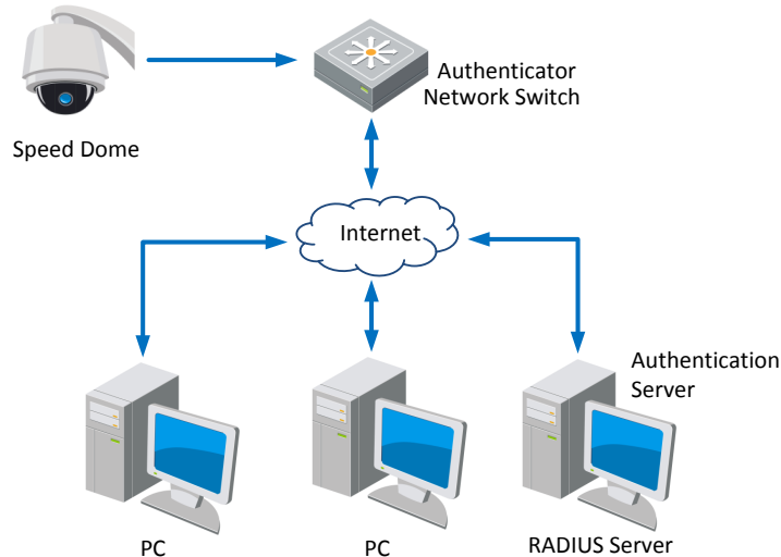
Figure 6-20 Protected LAN
